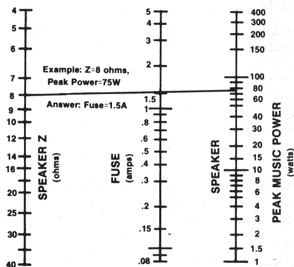
Fig. 3.8 Fuse Selector Nomograph for Loudspeaker Protection
