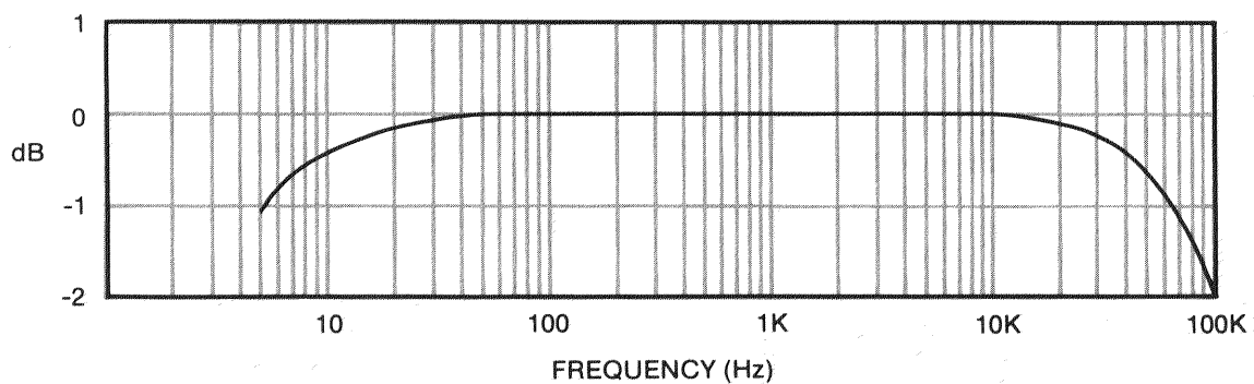
Fig. 2.7 Frequency Response
