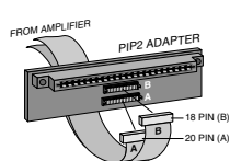
Fig. 8.1 PIP2 Adaptor Connection
