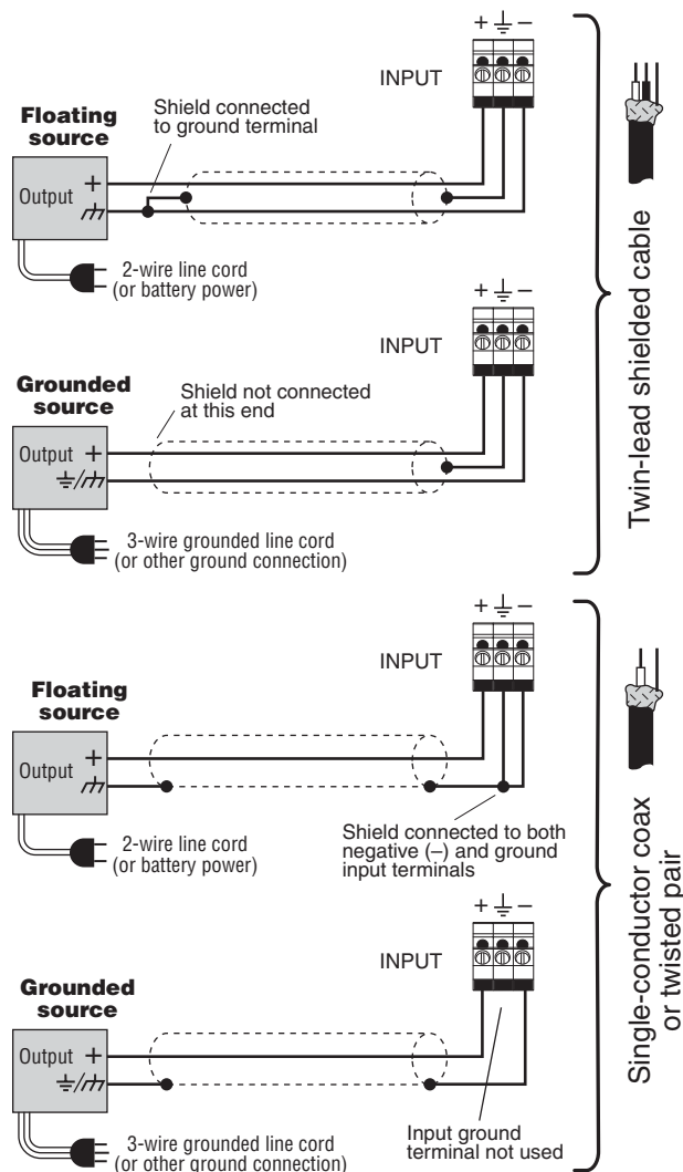
Fig. 3.9 Unbalanced Input Wiring
