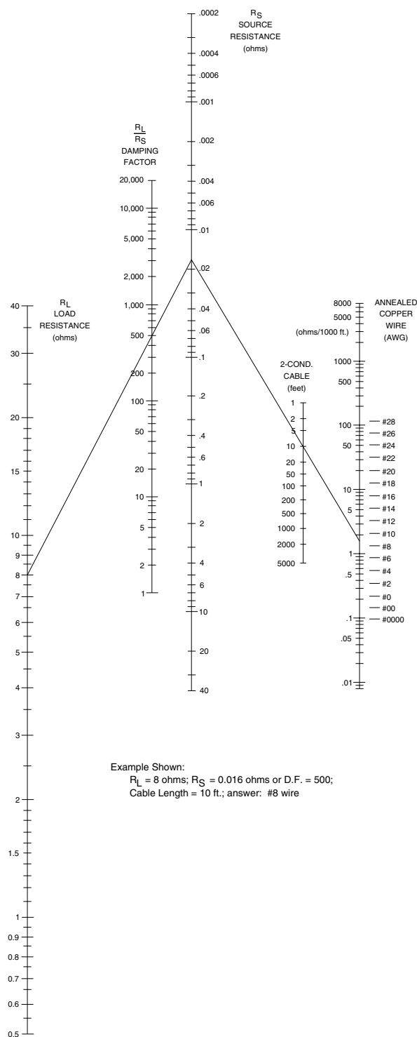
Fig. 3.14 Wire Size Nomograph
