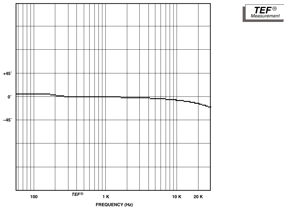
Fig. 6.12 Typical Phase Response
