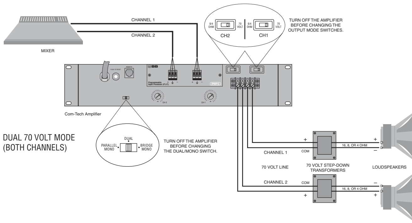
Fig. 3.5 Wiring for Dual 70-Volt Mode
