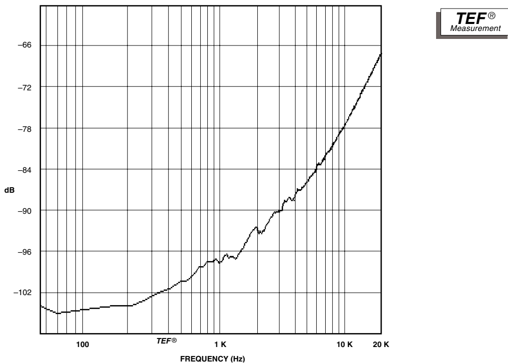
Fig. 6.13 Typical Crosstalk
