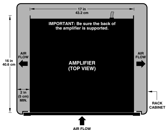
Fig. 3.2 Top View of a Rack-Mounted Unit
