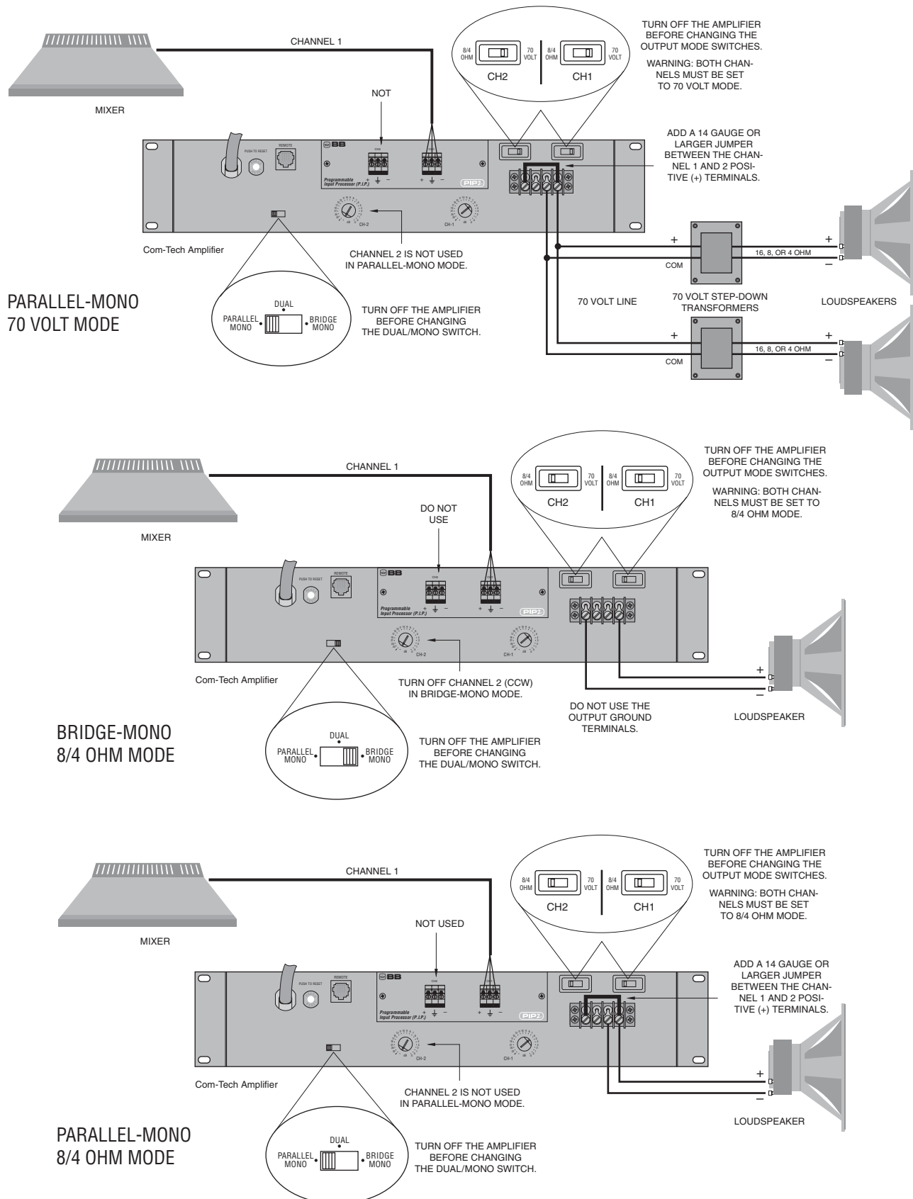
Fig. 3.7 Wiring for Parallel-Mono 70-Volt, Bridge-Mono 8/4-Ohm and Parallel-Mono 8/4-Ohm Modes
