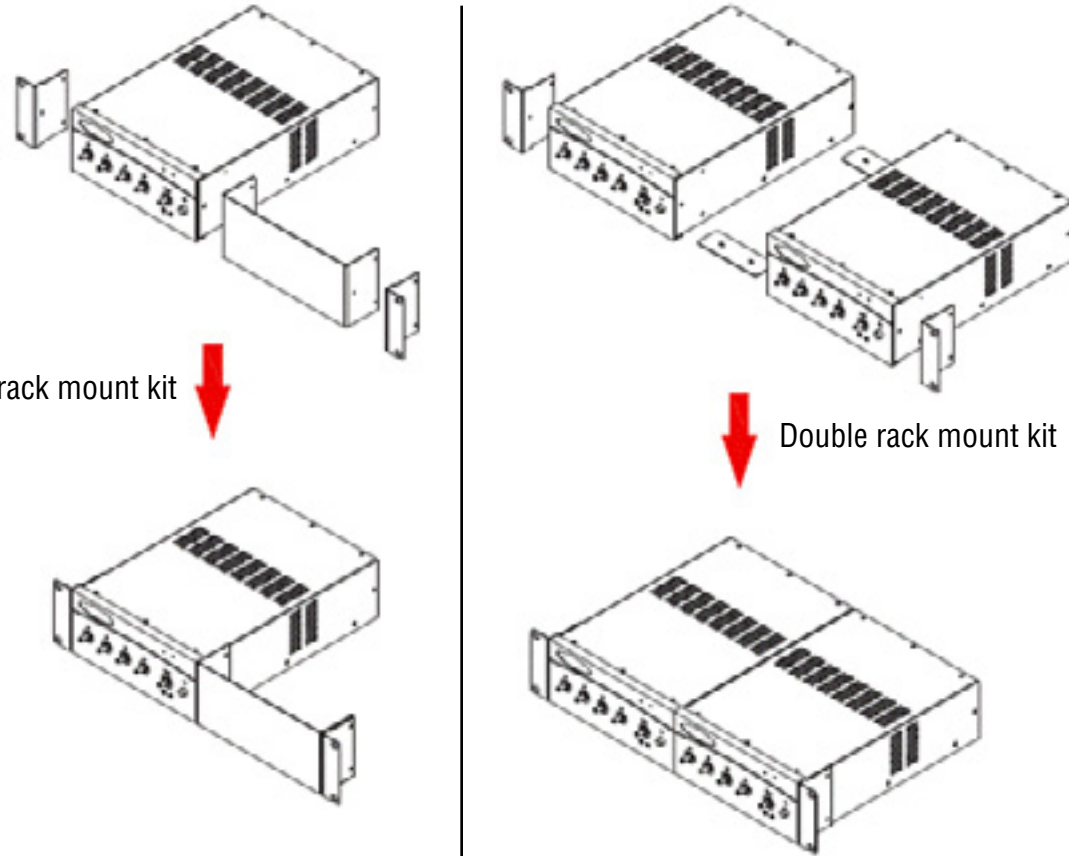
Figure 2.2 How to Connect Rack Ears (Not to Scale)
