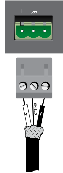
Figure 2.7 Connections to the Preamp Output Connector
