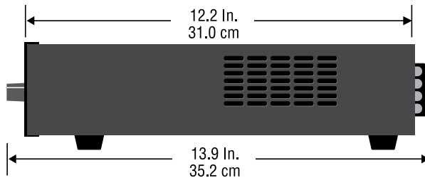
Figure 2.1 Dimensions
