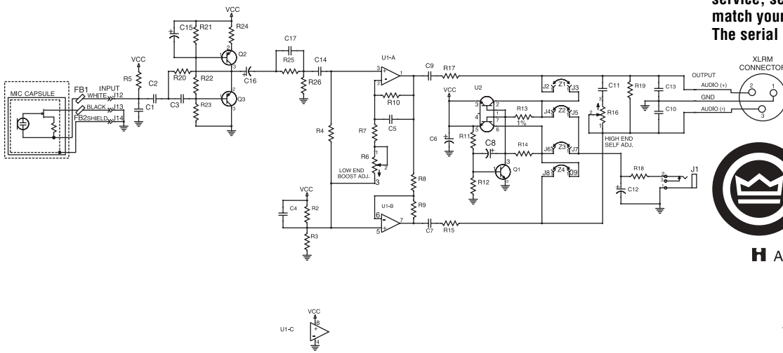
LM-201/LM-201L Schematic
