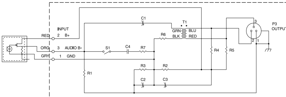
PZM-6D Schematic
